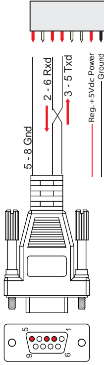
RS-232 communication / power connection
